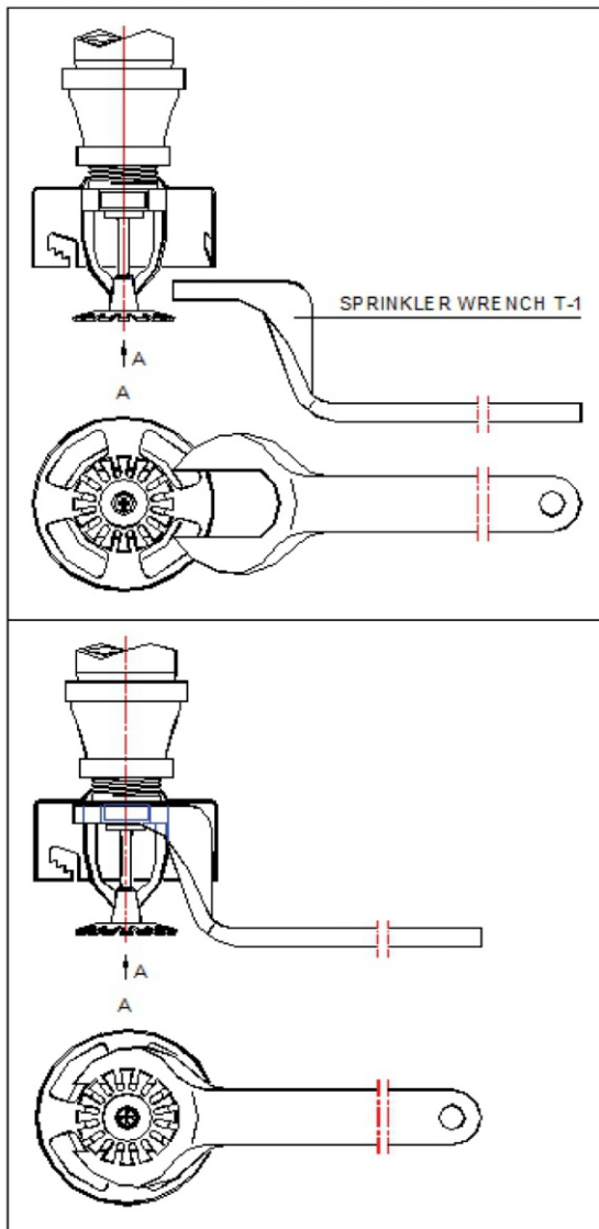
FIGURE C : SPRINKLER WRENCH SELECTION & USE
