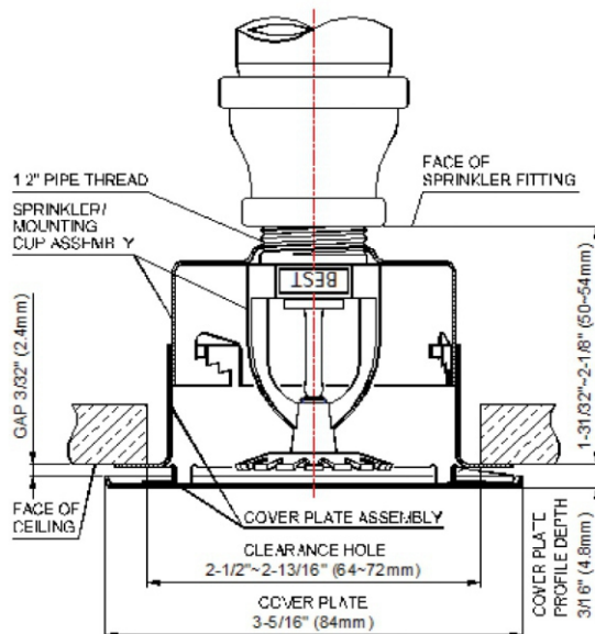
FIGURE E : MODEL BT007/BT008 CONCEALED PENDENT SPRINKLER TYPICAL INSTALLATION
