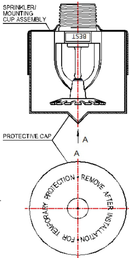
FIGURE D : PROTECTIVE CAP
